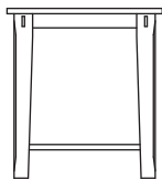
End Table TBE022A 22"W x 22"D x 24"H
