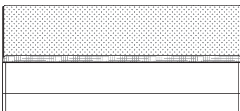
Console Table TBN028A 54"W x 16"D x 33"H
