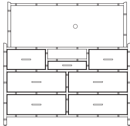
Queen TV/Stand Dresser TVD019A 62"W x 22"D x 60"H
