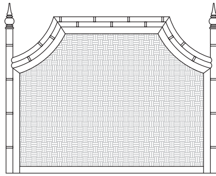
Queen Headboard QHB035A 62"W x 2 1/4"D x 50"H
