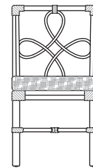
Dining Chair CHD026A 18"W x 19"D x 34"H
