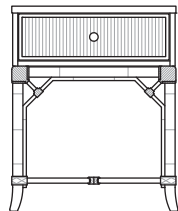
Twin Nightstand NST098A 24"W x 20"D x 30"H
