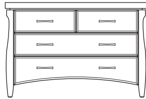
Queen Dresser DSR062A 48"W x 20"D x 32"H
