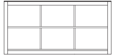
Bookcase BKC000A 60"W x 21 5/8"D x 30"H
